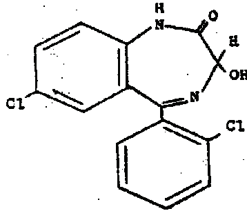
Figure 1: Lorazepam Structural Formula
