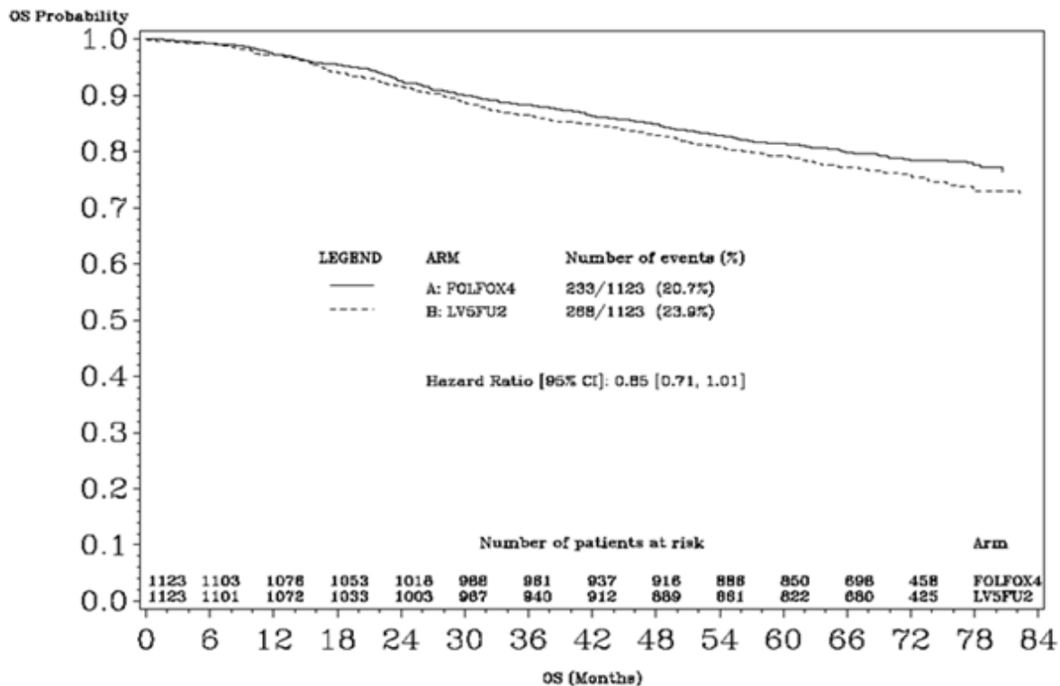
Figure 2. Kaplan-Meier OS curves for the comparison of Oxaliplatin and infusional 5-FU/LV combination and infusional 5-FU/LV alone for the ITT population.
