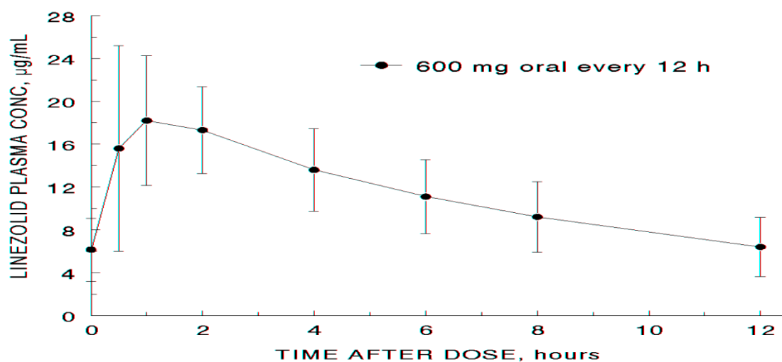
Figure 1. Steady-State Linezolid Plasma Concentrations in Healthy Adults Following Oral Dosing of 600 mg (Tablets) Every 12 Hours (Mean \pm Standard Deviation, n=16)
