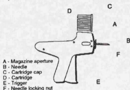
Figure 3 Diagram of the implanter and cartridge.
