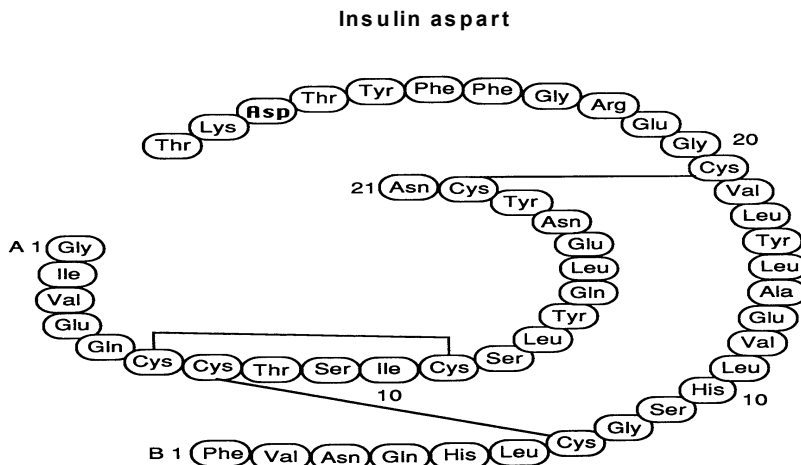
Figure 2 Structural formula of insulin aspart
