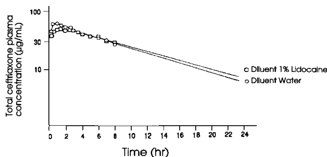
Figure 3 - Mean total ceftriaxone plasma concentration-time profiles after single intramuscular doses
