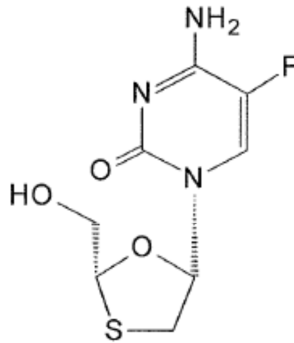
EMTRICITABINE
