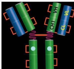
Figure 1 - Schematic Representation of the Structure of Alirocumab*
