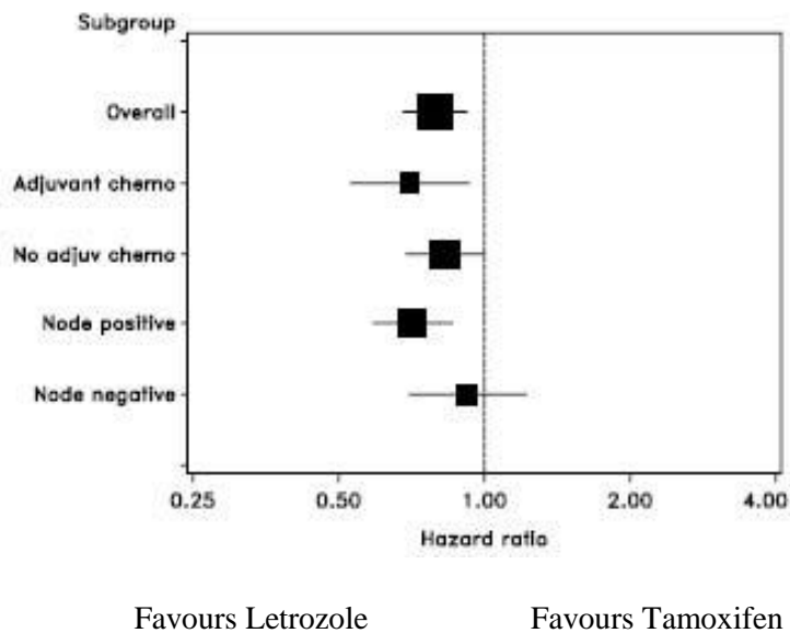
Figure 1: Forest plot for DFS by subgroup (median follow-up of 26 months)
