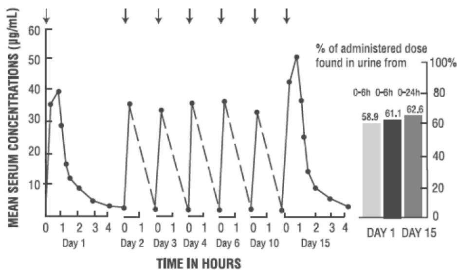
Figure 5 - Mean serum concentrations and urinary excretion data of cefotaxime infused intravenously over 30 min. as a single dose of 1.0 g, every 6 hours for 14 days in 16 healthy male volunteers.
