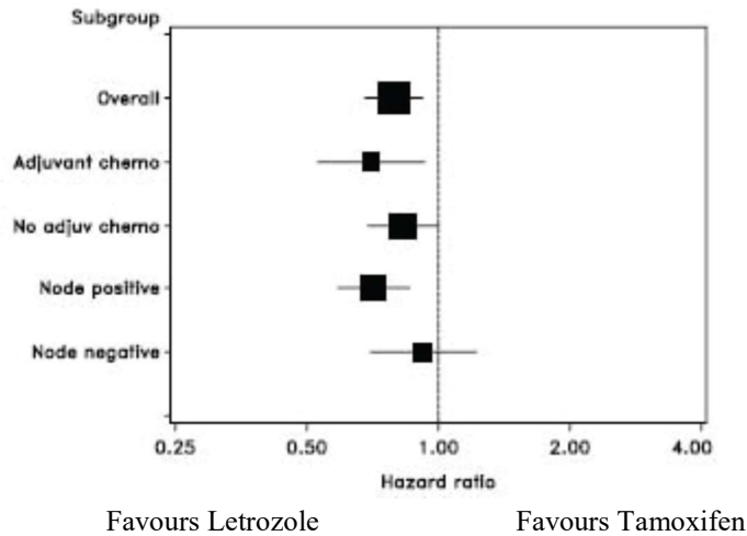
Figure 1: Forest plot for DFS by subgroup (median follow-up of 26 months)
