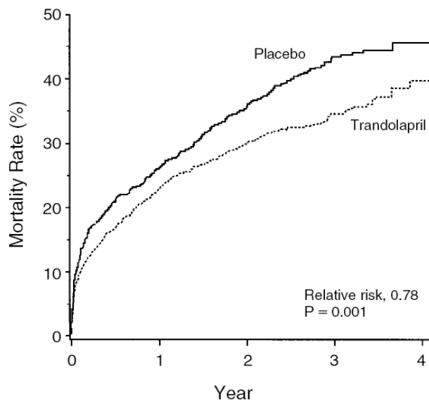
Figure 1: Cumulative Mortality from All Causes among Patients Receiving Trandolapril or Placebo
