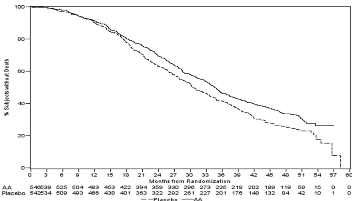
Figure 3: Kaplan Meier Survival Curves of Patients Treated with Either Abiraterone Acetate or Placebo in Combination with Prednisone plus GnRH Agonists or Prior Orchiectomy (Final Analysis; ITT Population)
