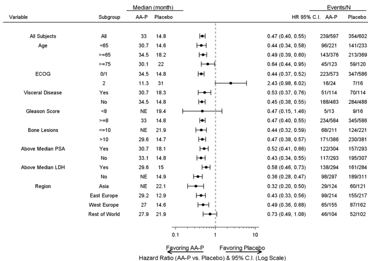
Figure 8: rPFS by Subgroup; ITT Population (Study PCR3011)
