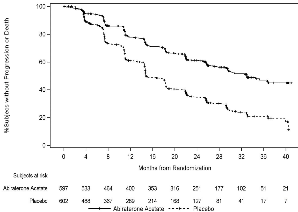
Figure 7: Kaplan-Meier Plot of rPFS; ITT Population (Study PCR3011)
