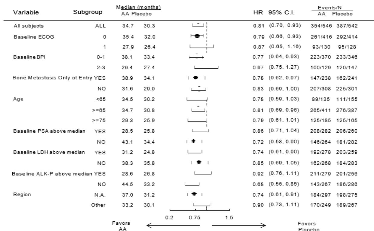
Figure 4: Overall Survival by Subgroup (Final Analysis) (ITT Population)
