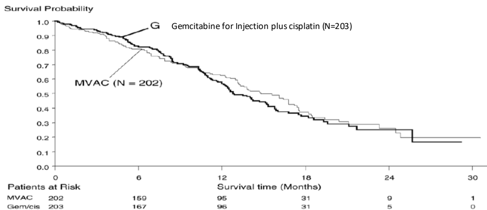
Figure 3: Kaplan-Meier Survival Curve in Gemcitabine for Injection (gemcitabine hydrochloride) plus Cisplatin versus MVAC Bladder Cancer Study (N=405)
