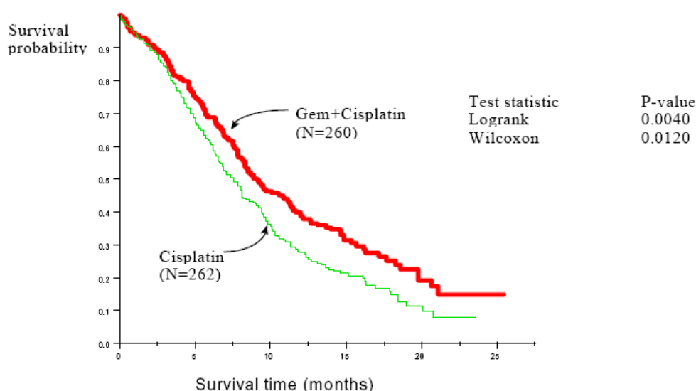
Figure 2 Kaplan-Meier Survival Curves - Gemcitabine for Injection (gemcitabine hydrochloride) plus Cisplatin versus Cisplatin in Non-Small Cell Lung Cancer
