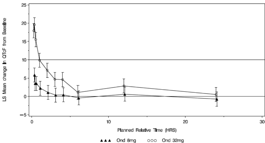
Figure 1: LS Mean Difference (90% CI) in QTcF Interval Between Treatment and Placebo Over Time
