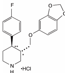
paroxetine hydrochloride
