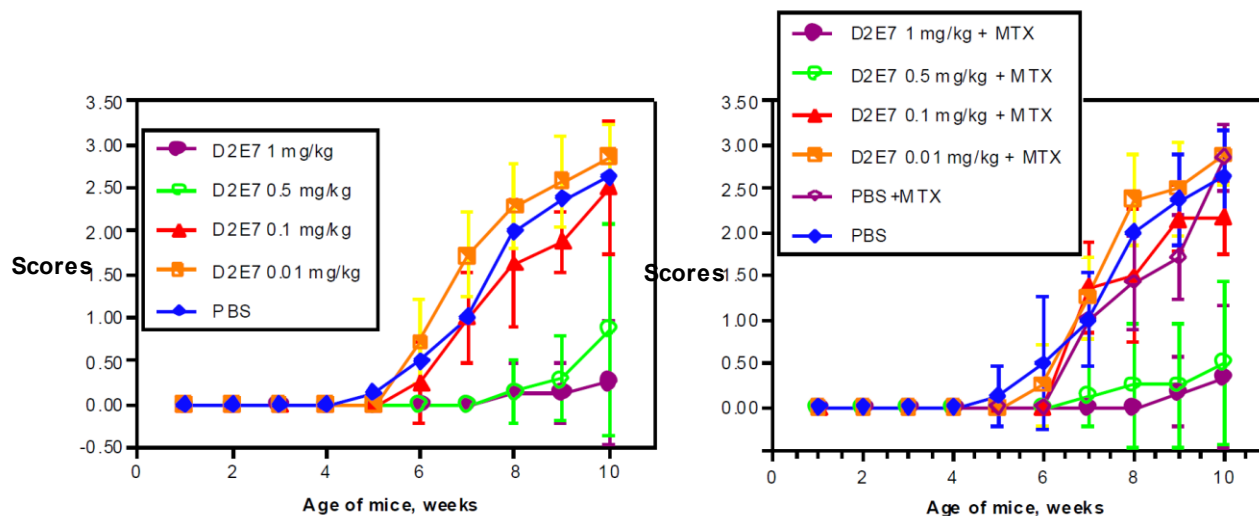
Figure 12. Mean Arthritic Scores of Study Groups During the Study Period
