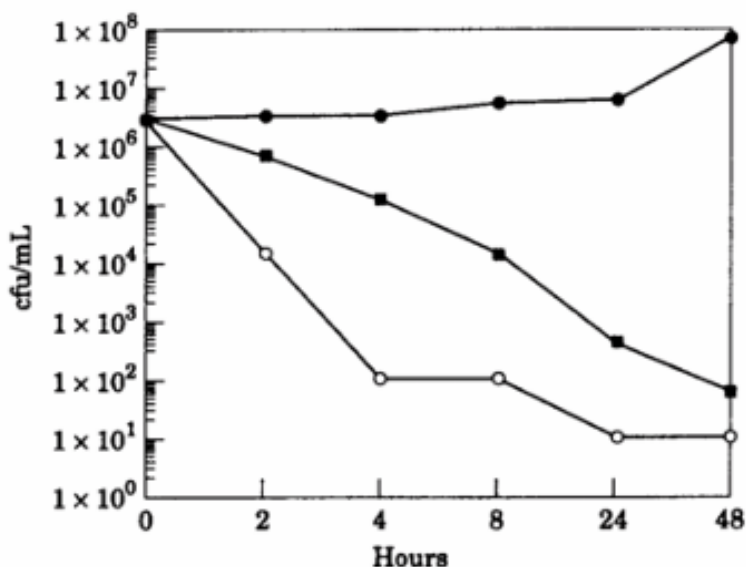
Figure 6: Kill kinetics of clarithromycin and 14-OH-clarithromycin against H. pylori strain 2597 at 8 x MIC and at pH 8.0. A flask was inoculated to produce a starting inoculum of approximately 10 6 cfu/mL. The flask was then incubated in an anaerobe jar with CampyPak® and shaken gently at 37 °C. Counts were done at 0, 2, 4, 8, 24, and 48 h in physiological saline after 72 h incubation. ●, No antimicrobial; ○, clarithromycin (0.12 mg/L); x, 14-OH-clarithromycin (0.24 mg/L).
