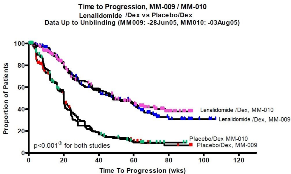
Figure 2: Kaplan-Meier Estimate of Time to Progression
