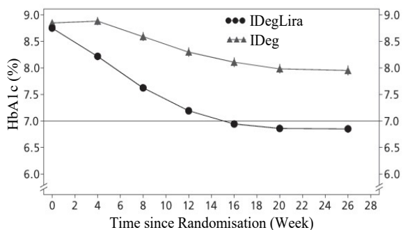
IDegLira=Xultophy®, IDeg=insulin degludec Figure 6: Mean HbA 1c (%) by treatment week in patients with type 2 diabetes mellitus inadequately controlled on basal insulin (Trial 3912, DUAL II)
