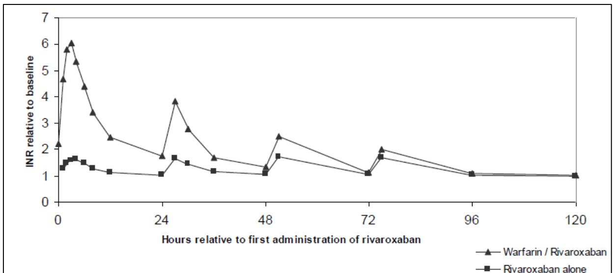
Figure 2: INR prolongation: Relative prolongation expressed as median of ratio to baseline with warfarin/ rivaroxaban treatment and rivaroxaban alone, following last day of warfarin
