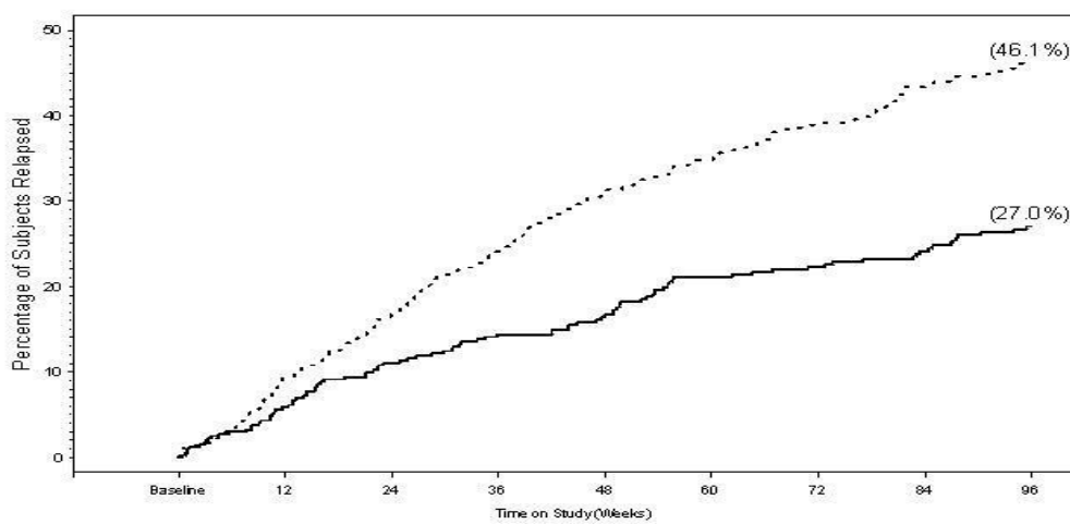
Figure 2 - Time to First Relapse in Study 1 (DEFINE) – Percentage of Patients Relapsed at 2 years
