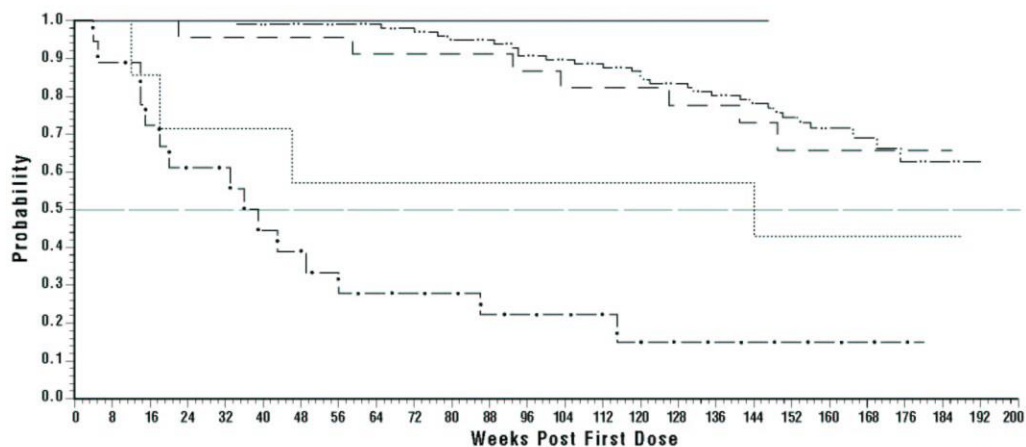
Figure 4: Kaplan-Meier estimate of overall survival since start of study by best response.
