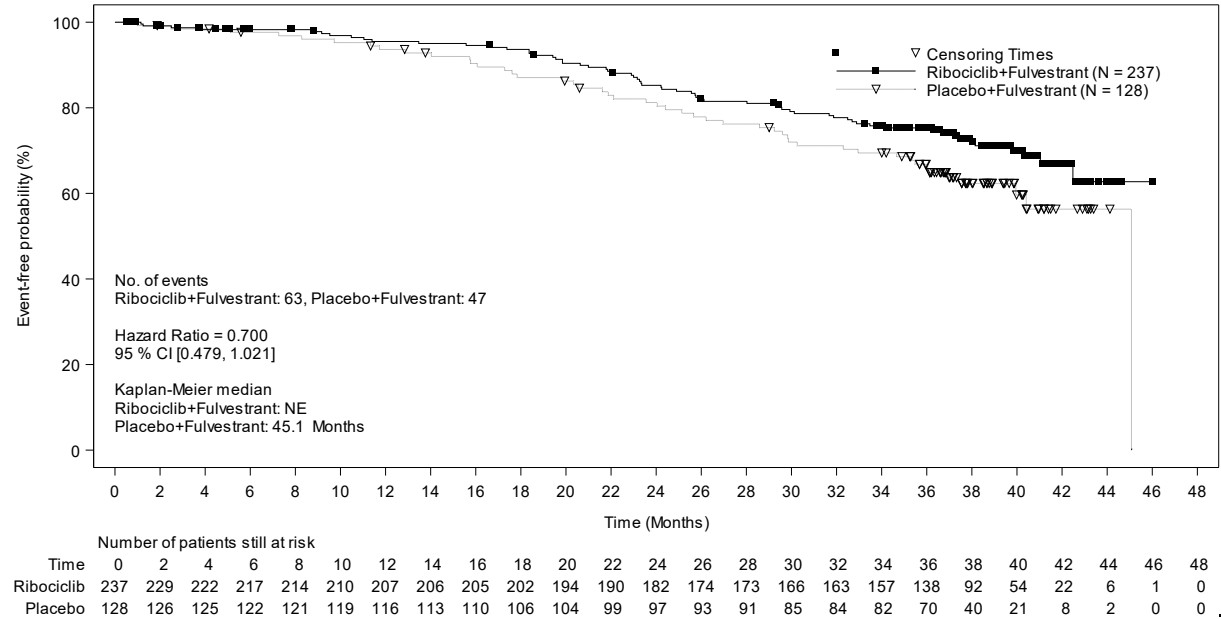
Figure 11 MONALEESA-3 (F2301) Kaplan Meier plot of OS for patients in first-line 1 setting (FAS) (03-Jun-19 cut-off)
