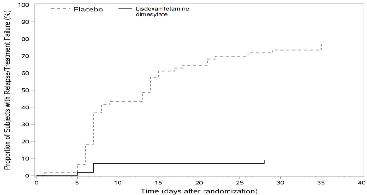
Figure 2 Kaplan-Meier Estimation of Proportion of Patients with Treatment Failure (adults)
