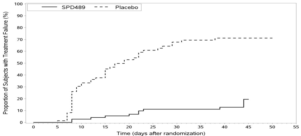
Figure 1 Kaplan-Meier Estimation of Proportion of Patients with Treatment Failure (children and adolescents)
