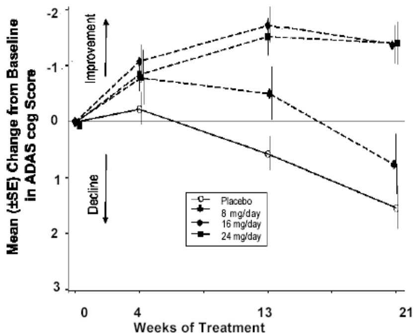
Figure 1: Time-course of the Changes from Baseline in ADAS-cog Score (ITT Population)
