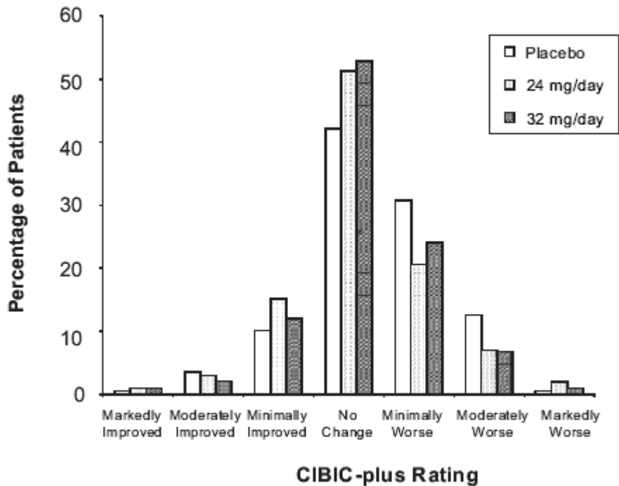
Figure 6: Distribution of CIBIC-plus Ratings Week 26 (ITT Population)
