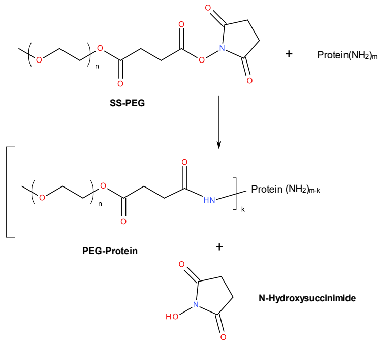
Figure 2: Reaction between SS-PEG and a Protein
