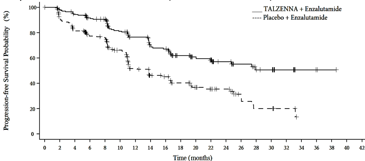
Figure 3. Kaplan-Meier Curve for rPFS in TALAPRO-2 (HRR Gene-mutated mCRPC)
