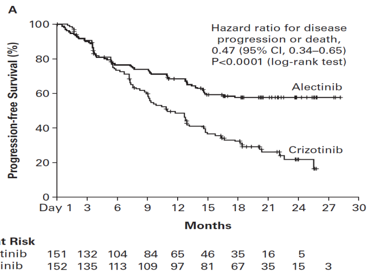
Figure 2 Kaplan Meier Plot of PFS as per central Independent Review Committee assessment from BO28984
