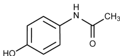
Figure 1 – Acetaminophen structure
