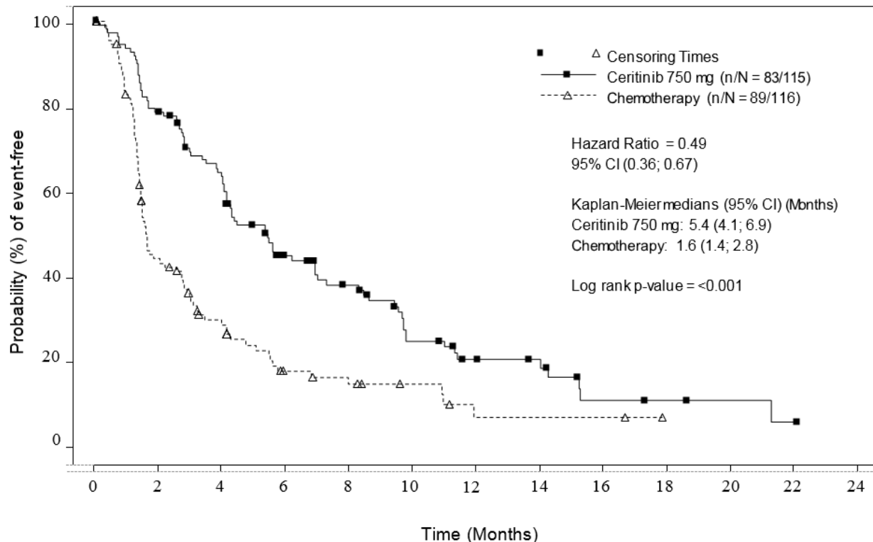
Figure 3 – Kaplan-Meier plot of progression-free survival as assessed by BIRC in Study A2303 (FAS, primary analysis)
