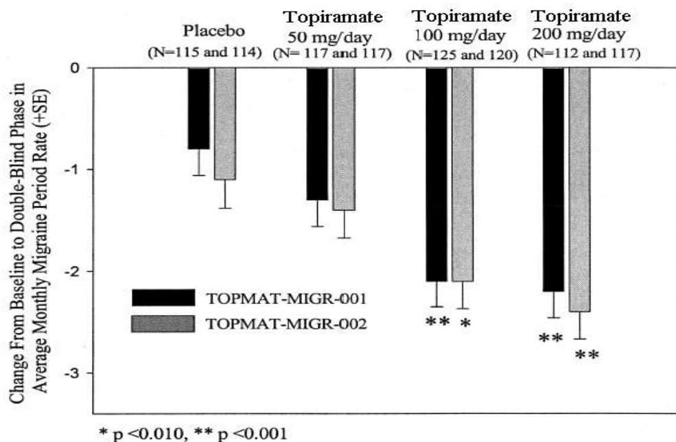
Figure 1: Reduction in 4-Week Migraine Headache Frequency (Studies TOPMAT-MIGR-001 and TOPMAT-MIGR-002)
