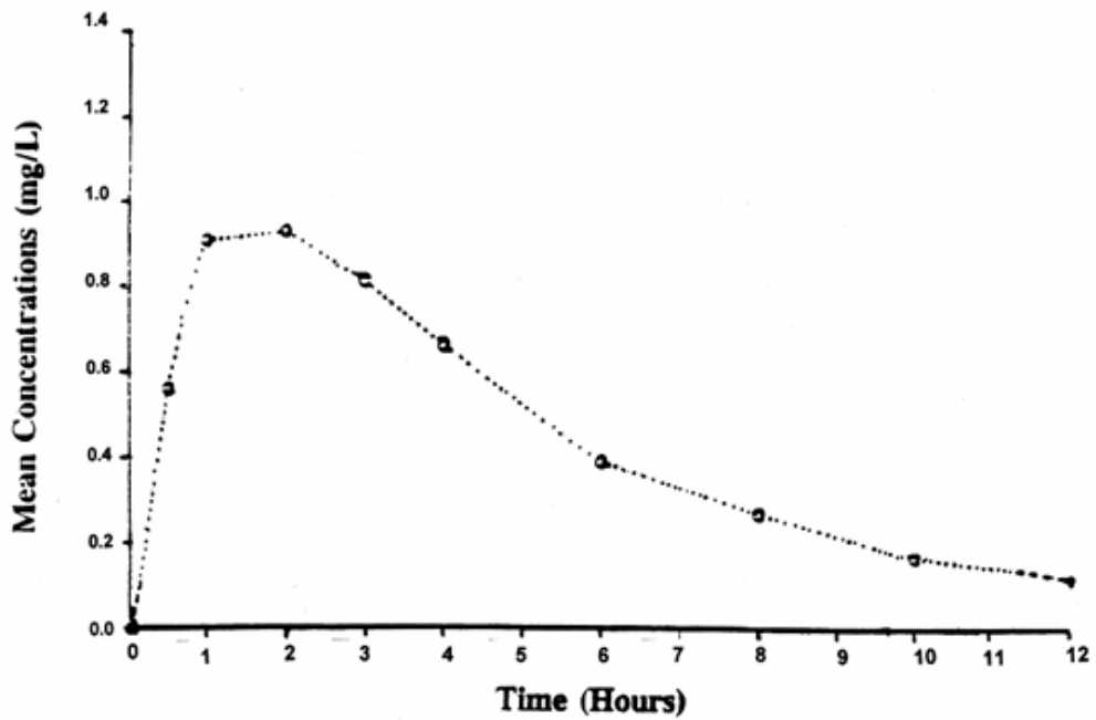
Figure 1: Plasma Clarithromycin Concentration (mg/mL) vs Time Following Oral Administration of a Single Dose of Clarithromycin 250 mg
