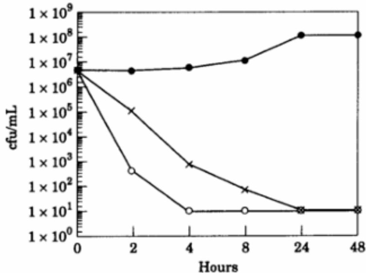
Figure 5: Kill kinetics of clarithromycin and 14-OH-clarithromycin against H. pylori strain 2597 at 8 x MIC and at pH 8. A flask was inoculated to produce a starting inoculum of approximately 10 6 cfu/mL. The flask was then incubated in an anaerobe jar with CampyPak® and shaken gently at 37 °C. Counts were done at 0, 2, 4, 8, 24,
