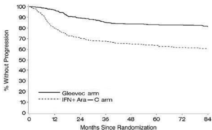
Figure 1 Time to progression (ITT principle)
